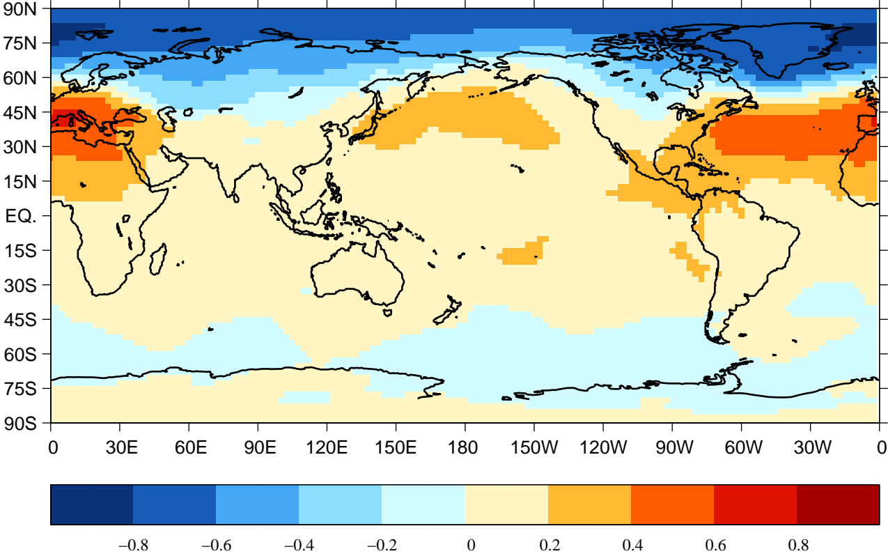
Northern Annular Mode (EOF1 NH SLP anomalies) 1948–Feb2005
