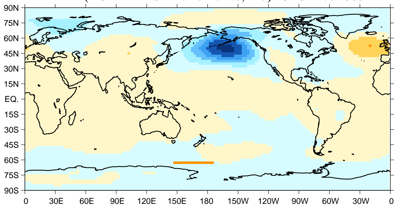
PNA (EOF2 NH SLP anomalies, mb) 1948–Feb2005
