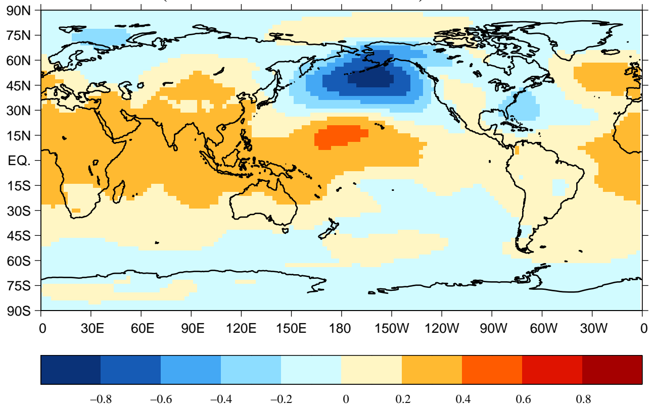
PNA (EOF2 NH SLP anomalies) 1948–Feb2005
