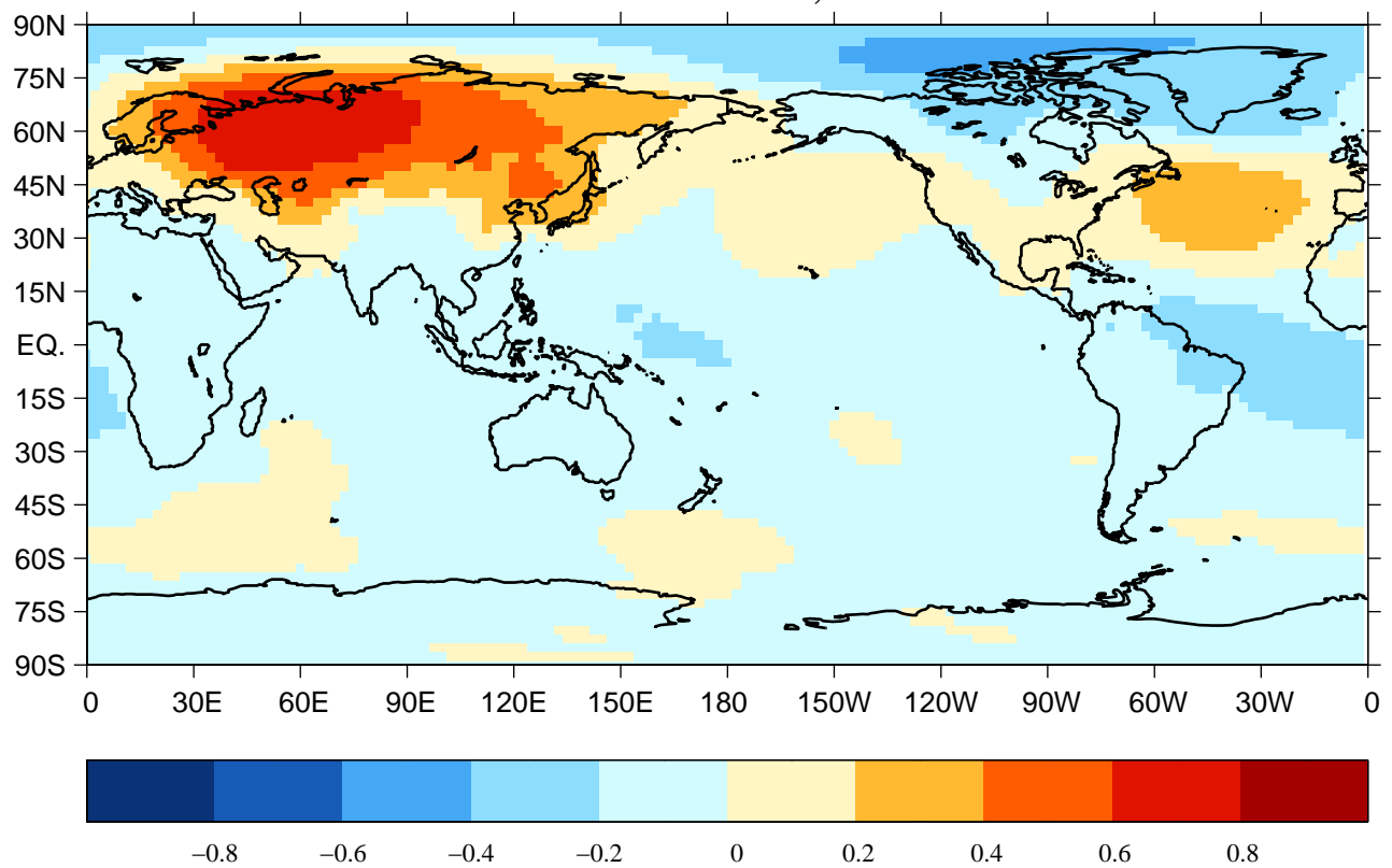
EOF3 NH SLP anomalies, 1948–June 2008
