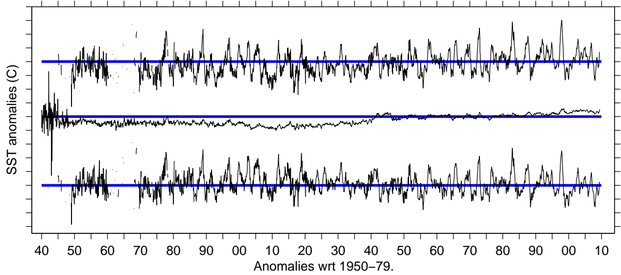
"cti-region", global-mean, "cti" (cti-region minus global mean) 1840-June2009
